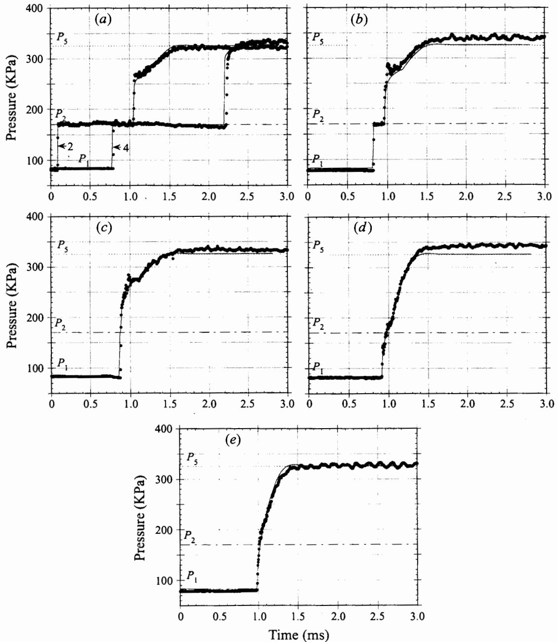
FIGURE 3. Typical results of the experimental results and their numerical simulations with a 40 mm long sample made of SiC having 10 pores per inch (i.e. sample I in table 1). The incident-shock-wave Mach number in this experiment was M_s = 1.378 (i.e. test number 1 in table 2). The pressure histories of the pure gas just ahead of the front edge of the porous material are shown in (a) and (b). The pressure histories of the gas occupying the pores of the porous material along the shock-tube sidewall and at its endwall are shown in (c), (d) and (e), respectively. The symbols represent the experimental results and the solid lines are the numerically predicted values. P_1 is the pressure ahead of both the incident and the transmitted shock waves, P_2 is the theoretical pressure which should have been reached behind the incident shock wave, and P_5 is the theoretical pressure which would have been reached had the incident shock wave reflected head-on from a solid endwall.
