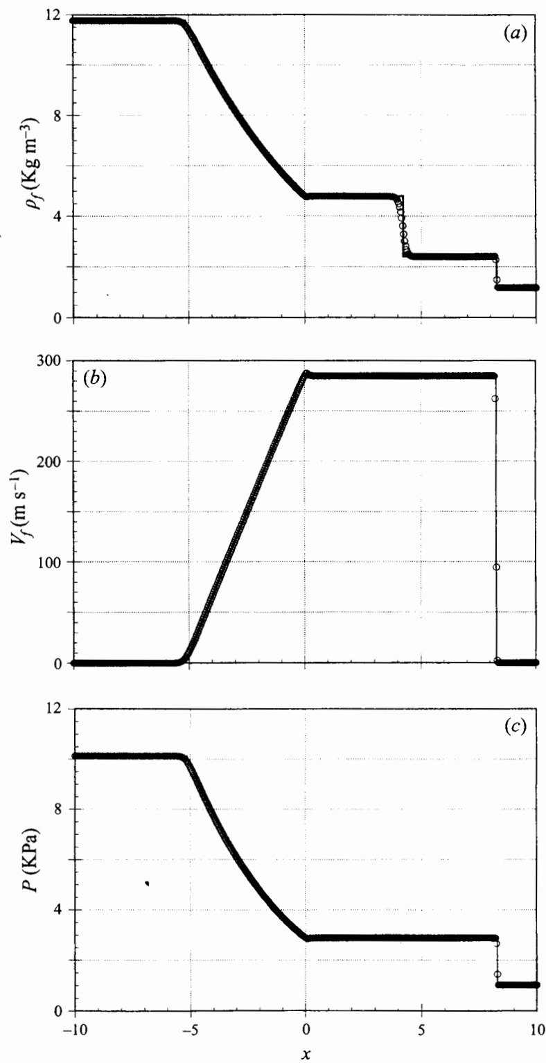
FIGURE 1. Comparison between the analytical solutions (solid lines) and the numerical predictions (open circles) of the classical one-dimensional shock tube problem: (a) density, (b) velocity and (c) pressure.
