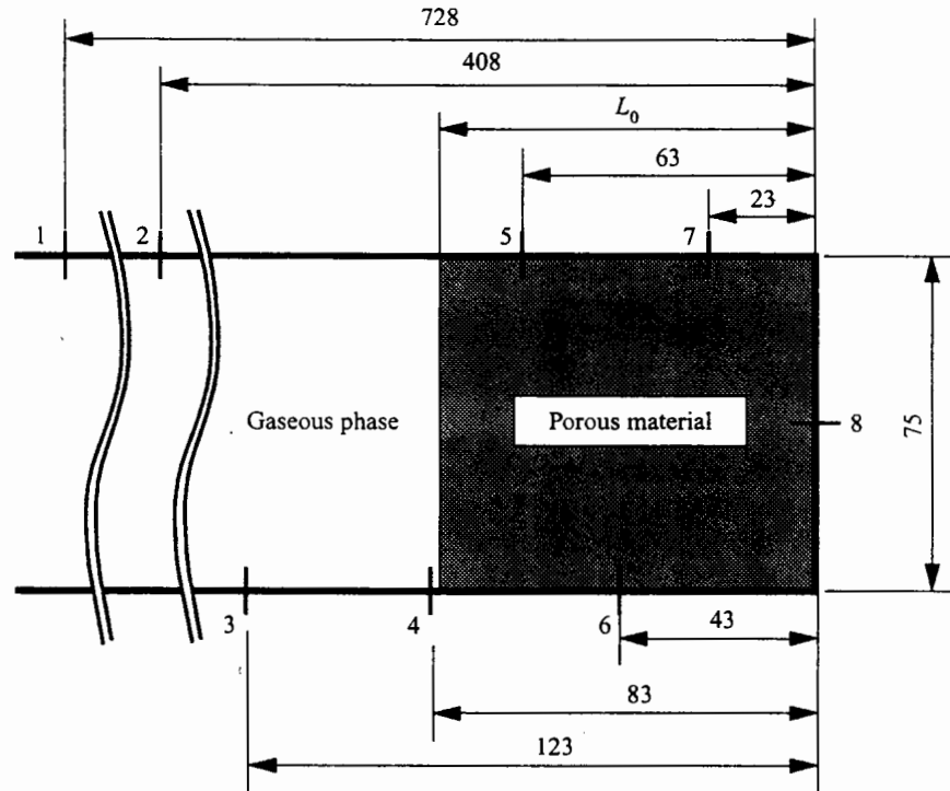
FIGURE 2. Schematic illustration of the experimental set-up and the locations of pressure transducers (numbered 1–8). All dimensions are in mm.
